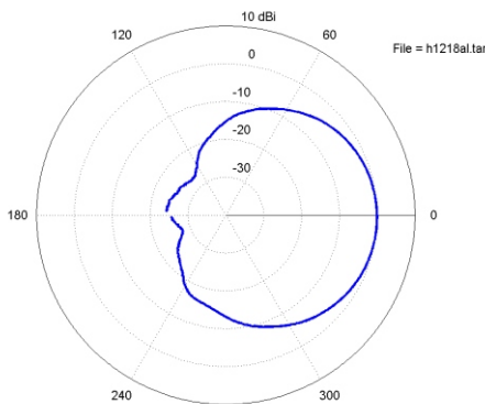
H-Plane patterns at 2450 Mhz
