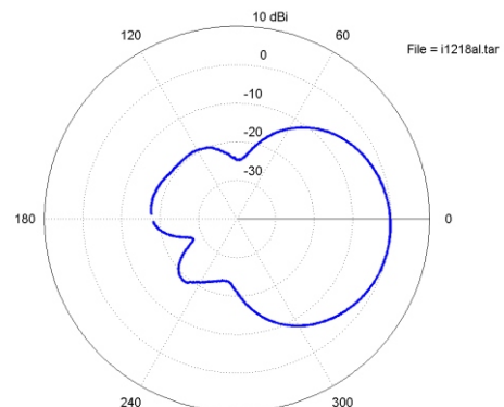
E-Plane patterns at 2450 Mhz
