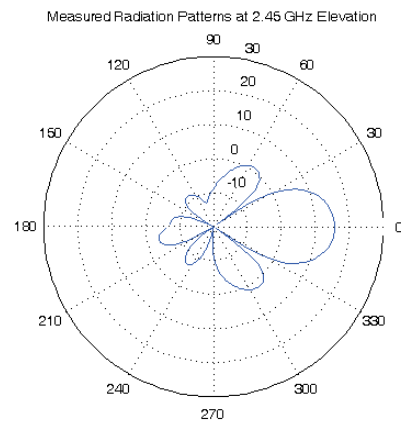
Radiation Pattern Elevation
