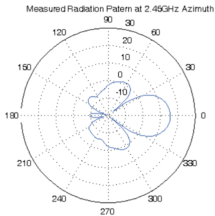
Radiation Pattern Azimuth
