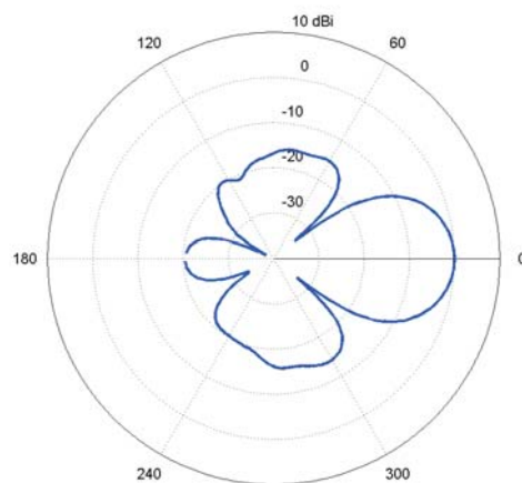
Azimuth at 2450 MHz (measured)
