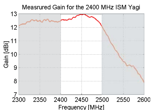
Gain
