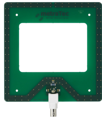
MidiPCB Antenna Art.-No.: 2200 0086
